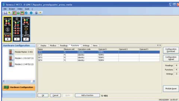
Fig.5.6 Functions definition on acquired temperatures
