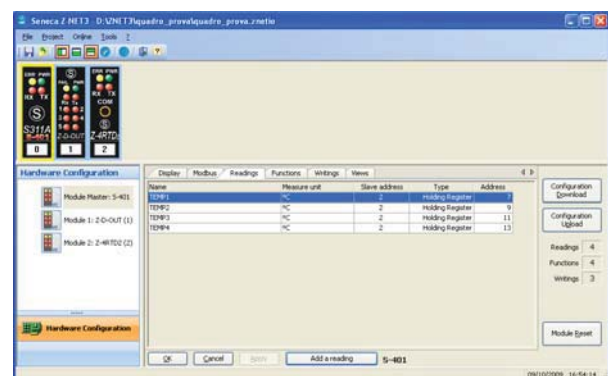
Fig.5.4. Readings definition from RTD
