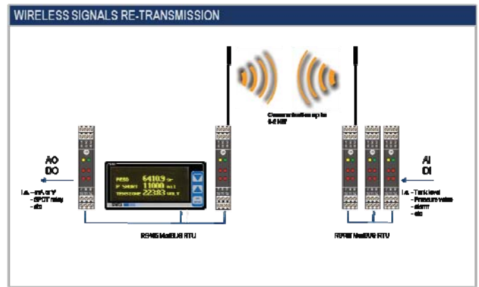
Fig. 5.10 Wireless Retransmission example
