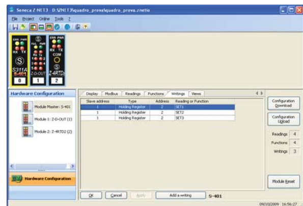
Fig. 5.8 Writings on alarm definition
